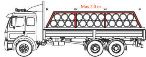
Appropriate use of tiedowns for a group of pipes
