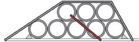
Correct secorement of front pipe in partial second tier
